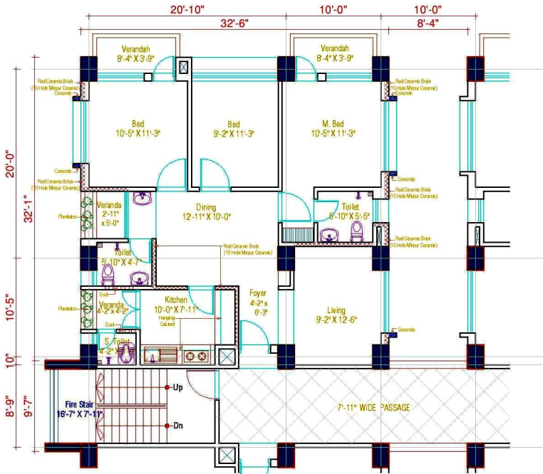
UNIT PLAN (TYPE B) UNIT AREA 1338 SFT
